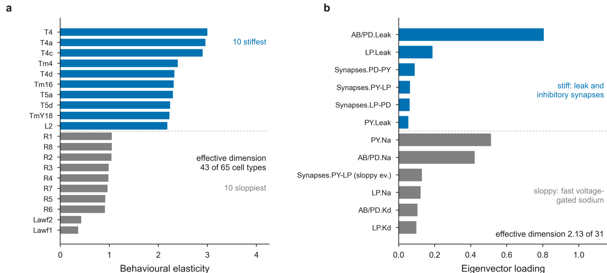
Figure 4: The fly visual model measured by parameter group, and the crustacean pyloric population. a Behavioural elasticity of the flyvis optic-lobe model by cell type, the ten stiffest (blue) and ten sloppiest (grey) of its 65 named types. The motion-detecting T4/T5 pathway and its medulla inputs are stiff; the photoreceptors and the lamina wide-field cells are sloppy. Which parameter group is probed matters as much as how many observables are recorded: the per-cell-type biases shown here give 43 of 65, the membrane time constants 5 of 65, the synaptic strengths 14 of 200, and the three groups measured jointly 14 of 330 sampled parameters, which is the figure comparable with the other systems here. b Eigenvector loadings of the Prinz–Marder pyloric conductance population under the same estimator, with the leak and inhibitory-synapse conductances stiff and the fast sodium conductances sloppy. This model is also the best conditioned in the study, with the response proportional to the perturbation across two decades of step size (ratio 0.498 for the biases). Curvature is the Gauss–Newton form H = J^T W J .
