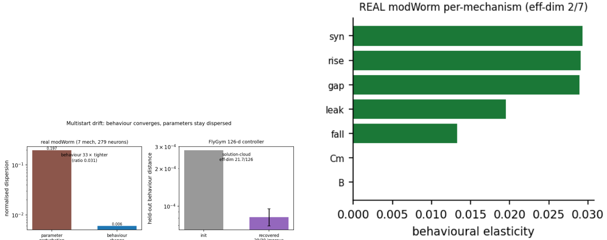
Figure 1: The behavioural-equivalence manifold, measured. a , Multistart drift: independent optimisations converge in behaviour while the recovered parameters remain dispersed (FlyGym 29/30 behavioural success, solution-cloud effective dimension 21.7/126; real modWorm behaviour approximately 30 \times less variable than its parameters), indicating a positive-dimensional manifold. b , Gauss–Newton behavioural curvature per biophysical mechanism on the full coupled real modWorm model (OpenWorm connectome, 279 neurons). The synaptic and gap-junction conductances and the synaptic rise time carry the curvature, whereas the membrane capacitance and the sigmoid gain are behaviourally flat, giving an effective dimension of 2 of 7: a small number of stiff directions and many sloppy ones.
