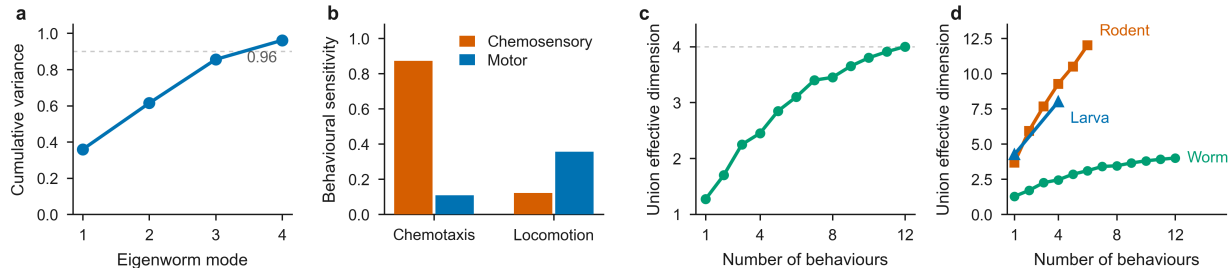
Figure 2: The identifiable subspace is the eigenworm space, tiled complementarily by behaviour, across phyla. a , Cumulative postural variance of real C. elegans posture (Open-Worm Movement Database, n=8432 frames) across eigenworm modes; four modes capture 0.96 of the variance (dashed line, 0.90). Two independently constructed worm models align with this empirical basis at \cos 0.77 (modWorm) and \cos 0.68 (BAAIWorm). b , Behavioural sensitivity to perturbation of the chemosensory (vermillion) and motor (blue) parameter classes, during food-directed chemotaxis and during plain locomotion in a weak gradient. Chemosensory parameters are stiff during chemotaxis but sloppy during locomotion (a 7.15\times context shift) and motor parameters show the reverse contrast, so distinct behaviours constrain distinct axes. c , Union effective dimension of the identifiable subspace as behaviours are added (real modWorm, twelve behaviours), saturating at 4 of 7 mechanism directions (dashed line) and leaving a residual degenerate core. d , The same increase with repertoire size in three phyla: nematode (green, 7 mechanisms), fly larva (blue, 10 parameters) and rodent (vermillion, 38 actuators). Absolute counts are not comparable across species because the models are parameterised differently; the structure is invariant.
