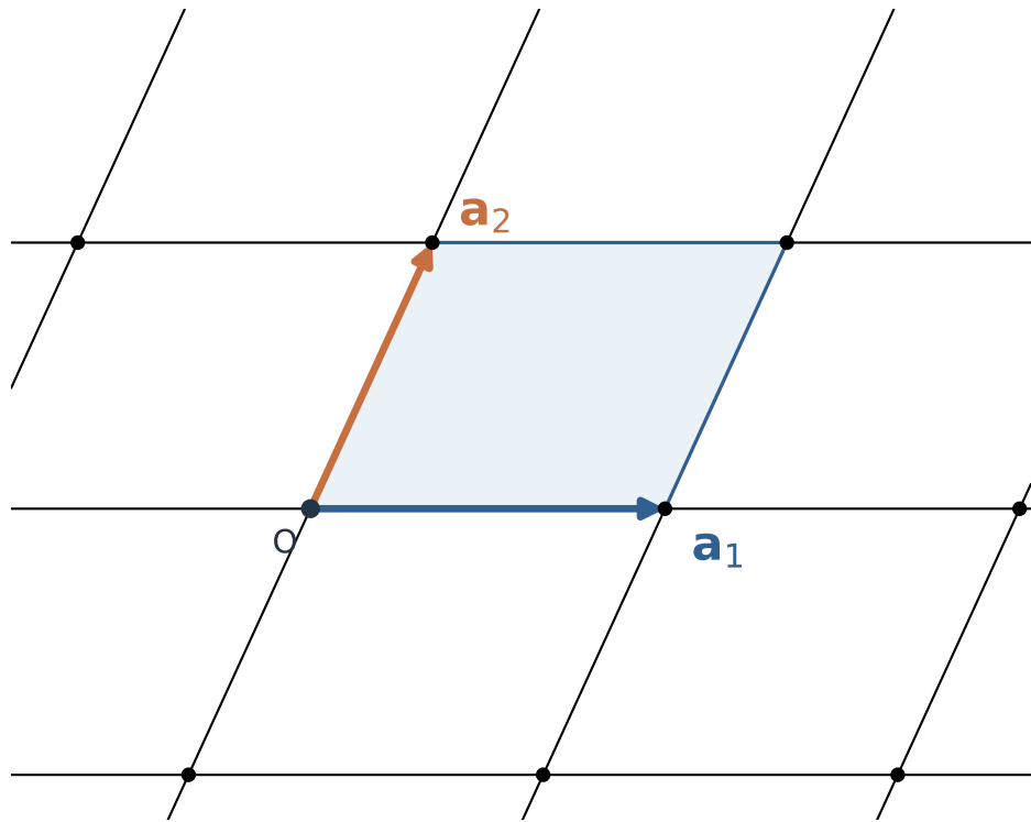
(a) Primitive lattice
