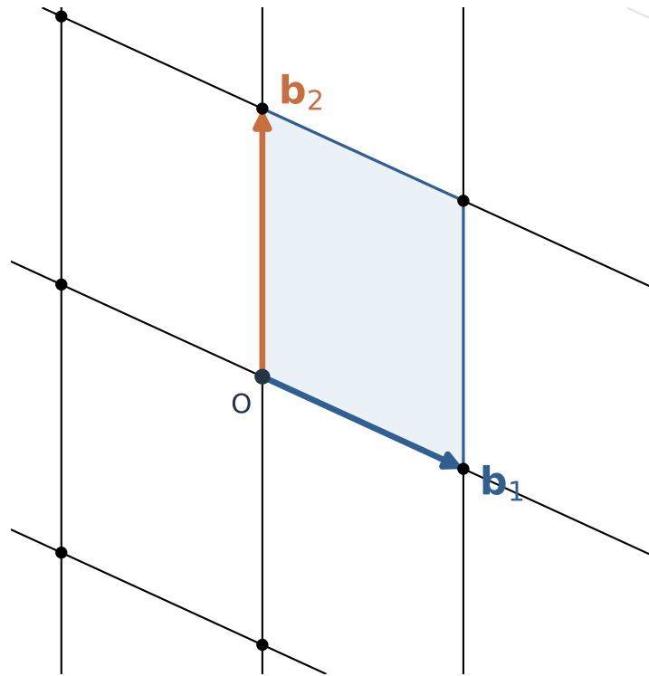
(b) Reciprocal lattice
