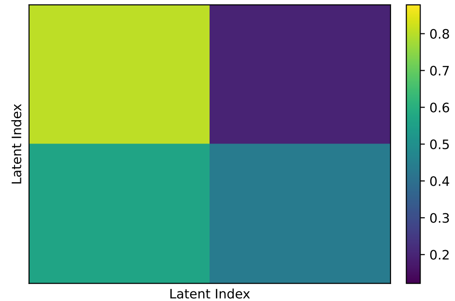
Normal Self-Attention
