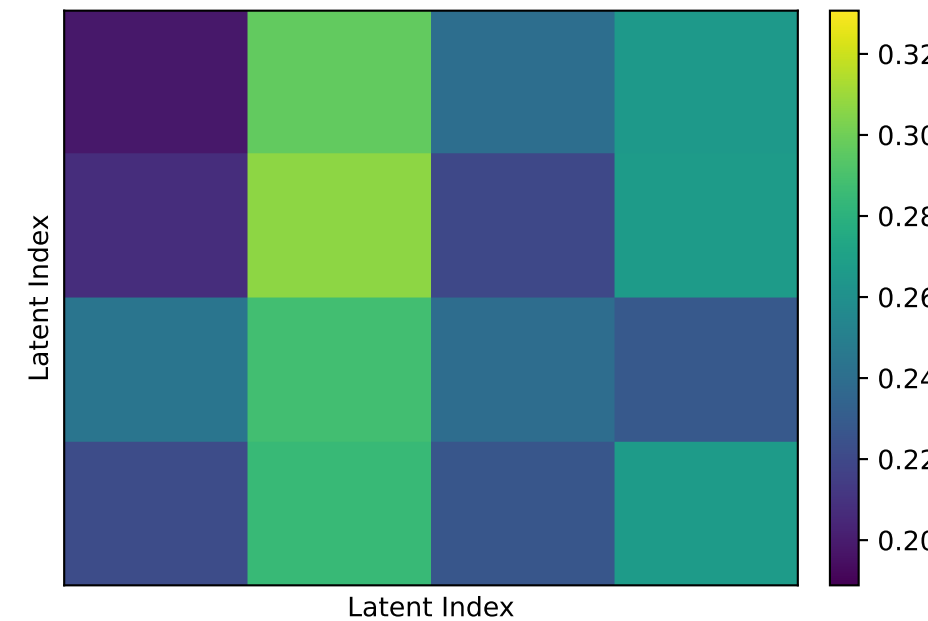
Abnormal Self-Attention
