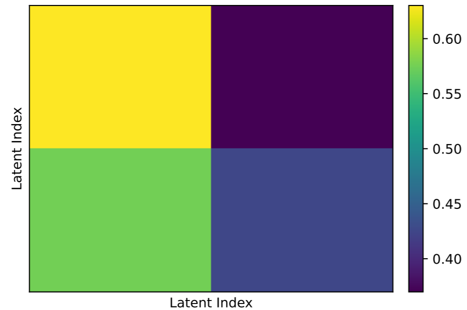
Normal Self-Attention
