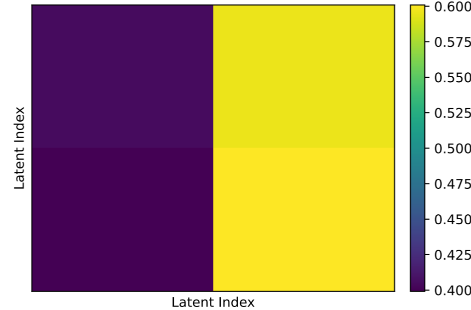
Normal Self-Attention
