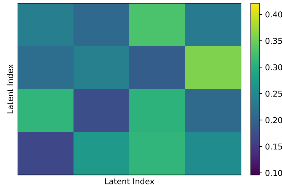
Abnormal Self-Attention
