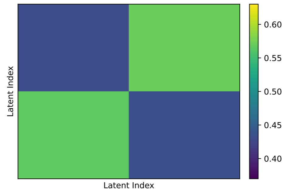
Abnormal Self-Attention
