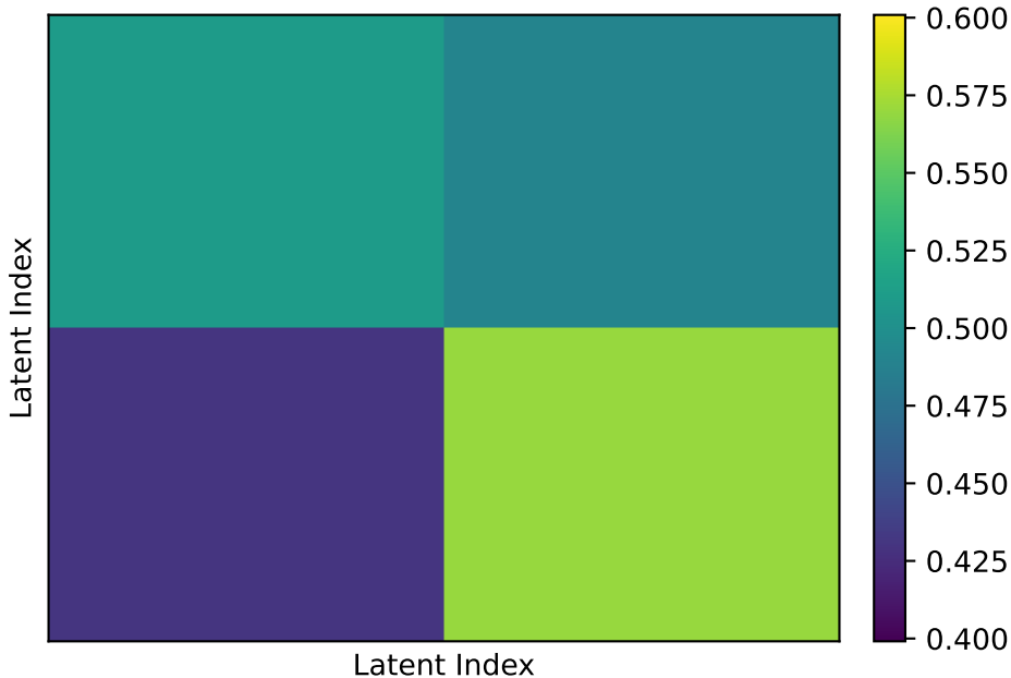
Abnormal Self-Attention
