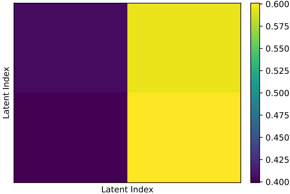
Normal Self-Attention
