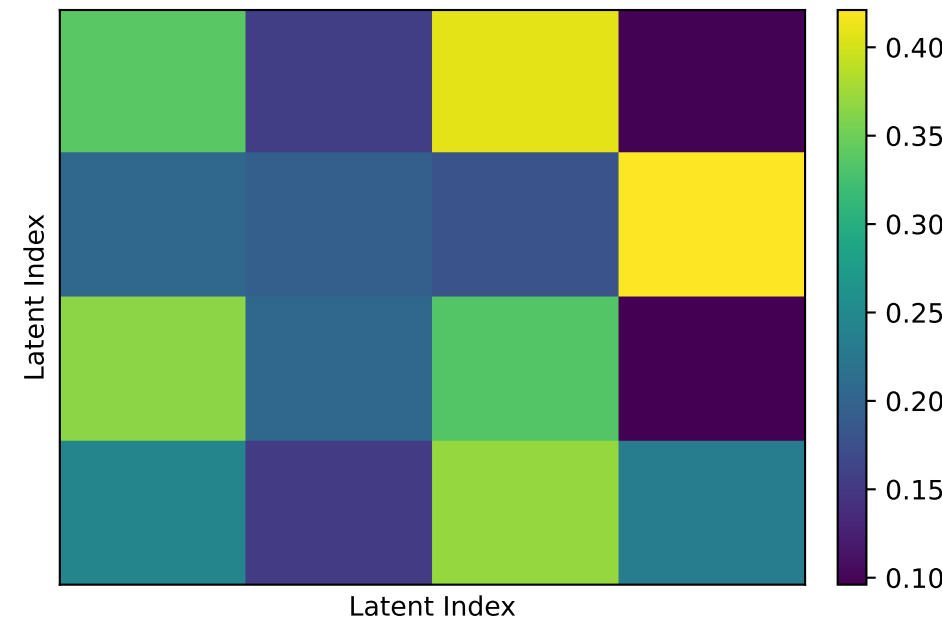
Normal Self-Attention
