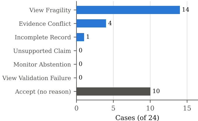
(b) Gate outcomes across all cases
