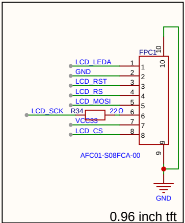
0.96 inch tft
