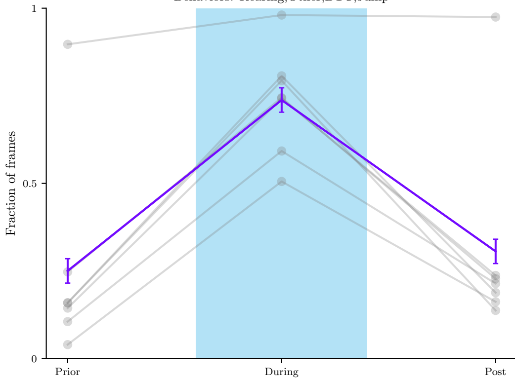
Change in behavior around laser epoch Behaviors: Rearing, Other, BTC, Jump
