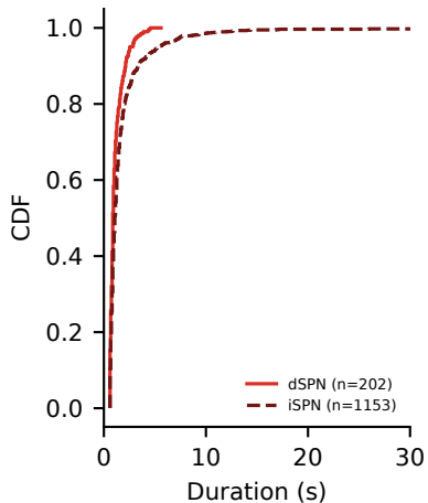
A Floor licking — Cocaine 5
