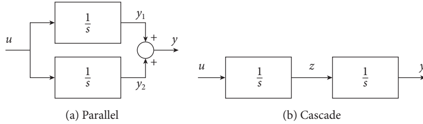
FIGURE 7.1. Block interconnections.
