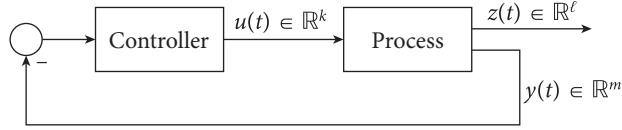
FIGURE 21.1. Linear quadratic regulation (LQR) feedback configuration.
