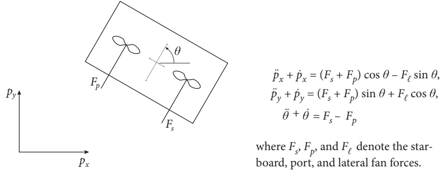
FIGURE 2.7. Hovercraft model.
