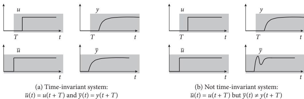
FIGURE 3.2. Time invariance: For an input u with output y , for every time shifted version \bar{u} of u there must exist an output \bar{y} that is a time shifted version of y .
