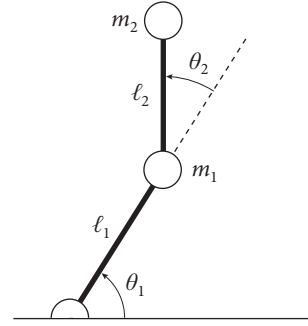
FIGURE 2.3. Two-link robot manipulator.
