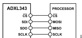
Figure 25. 4-Wire SPI Connection Diagram
