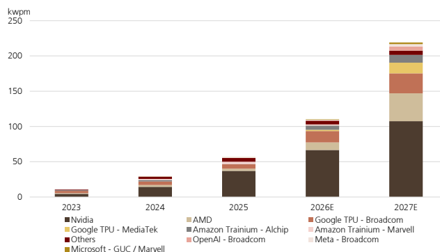
Figure 12: CoWoS demand from major customers
