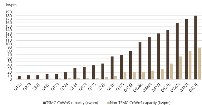
Figure 10: TSMC vs. non-TSMC CoWoS capacity
