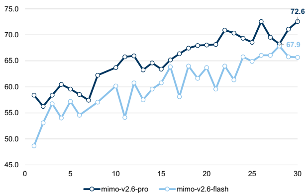
Exhibit 1: MiMo-V2.6-Pro/Flash scores on DeepSWE v1.1 benchmark by step (avg@3)
