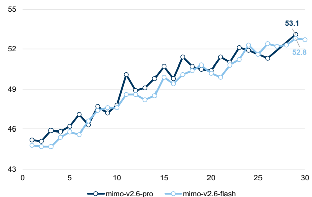
Exhibit 2: MiMo-V2.6-Pro/Flash scores on AutomationBench v1.0.6 benchmark by step (avg@3)
