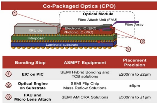
ASMPT Equipment Matrix – CPO Assembly Flow
