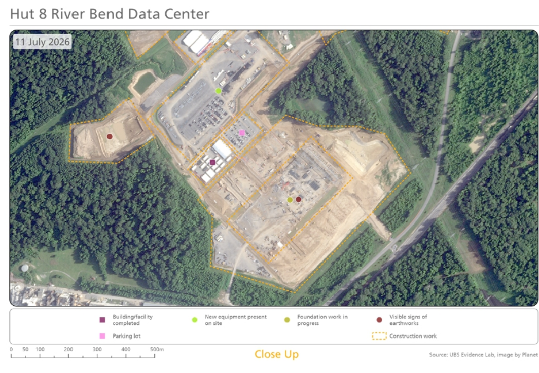
Figure 8: Hut 8 River Bend Construction Progress
