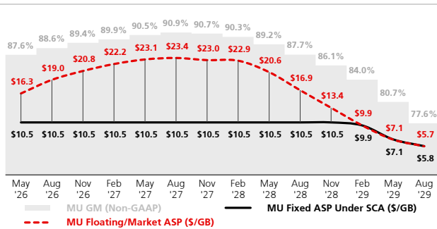
Figure 9: MU Fixed vs. Floating/Open Market ASP and Gross Margin Trends
