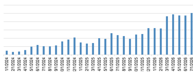
Figure 10: Chinese players' ESS battery exports to RoW (markets excluding China, the US and the EU) (monthly) (Unit: Gwh)
