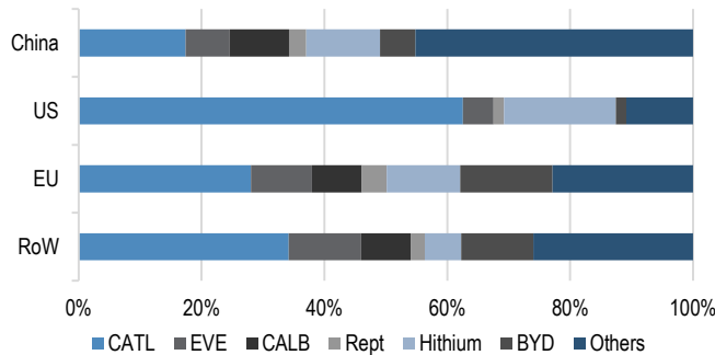
Figure 21: Chinese players' market share in each utility-scale ESS battery market (YTD)
