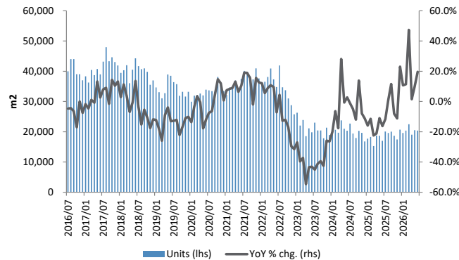
Figure 28: Rigid module boards: Production quantity (square meters)
