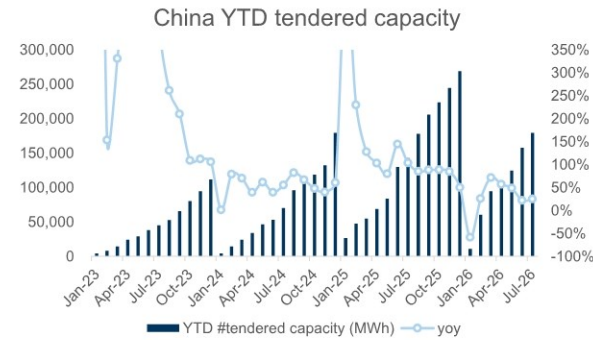
Exhibit 45: China: Total tendered ESS capacity was 179.2GWh in Jan-Jul 2026 (+25% yoy)
