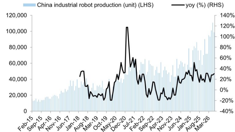
Exhibit 13: China industrial robot production +30% yoy/-11% mom in Jul (vs. past five years' seasonality of -5% mom)
