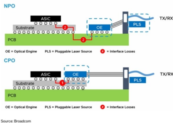
EXHIBIT 2: NPO places the optical engine on the PCB
