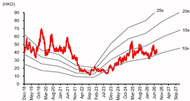
Fig. 4: AAC – P/E band
