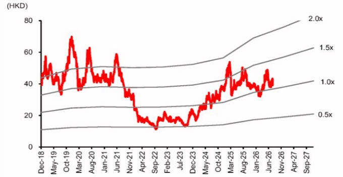
Fig. 5: AAC – P/B band
