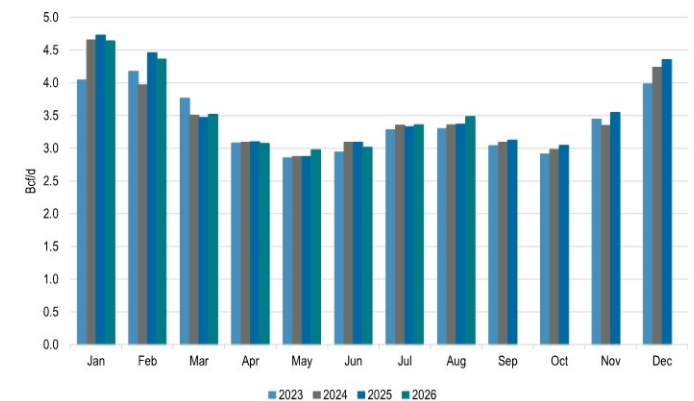
Figure 52: Pipe Loss Consumption (Bcf/d)
