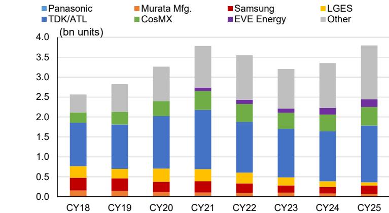
Laminated small size LiB shipment volume by supplier
