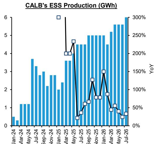
EXHIBIT 28: CALB - monthly production for ESS was 6.0GWh(33%YoY)
