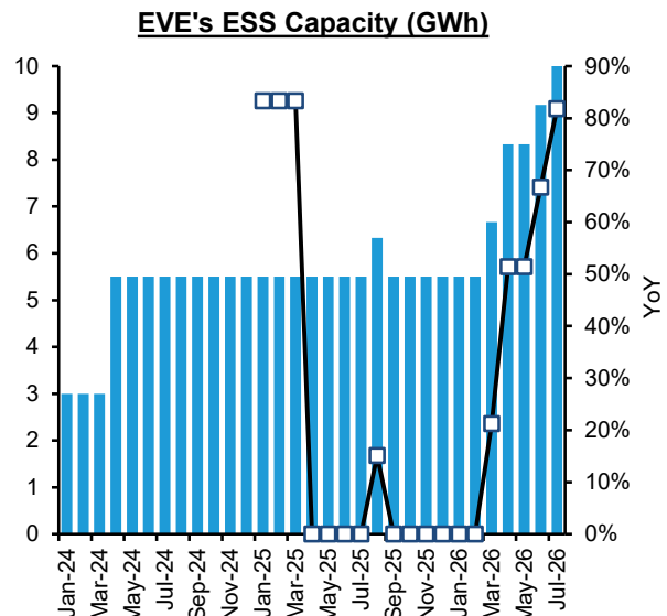
EXHIBIT 34: EVE – monthly capacity for ESS was 10.0GWh(82%YoY)
