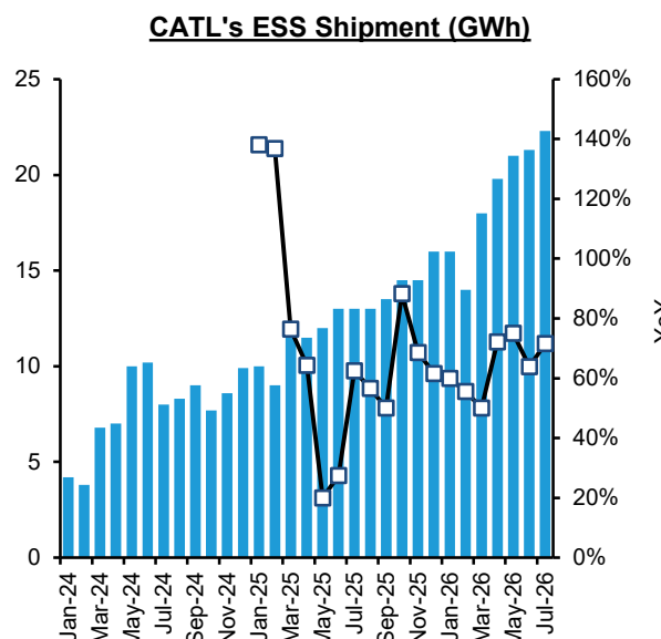
EXHIBIT 19: CATL - monthly shipment for ESS was 22.3GWh(72%YoY)
