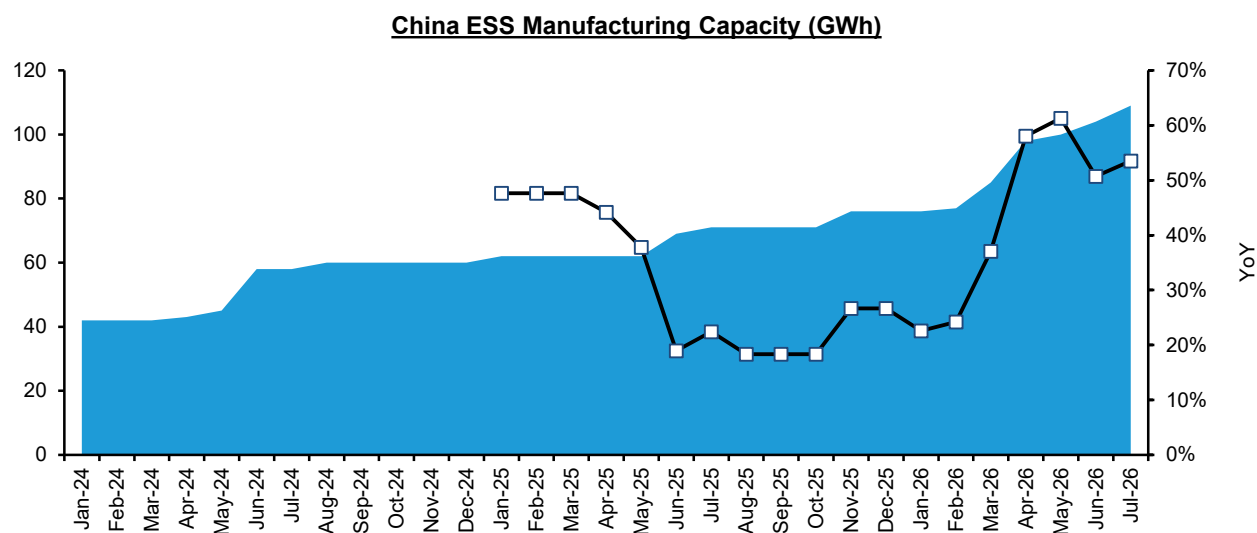
EXHIBIT 7: Monthly China ESS batteries manufacturing capacity was 109.0GWh (54%YoY, 5% MoM)
