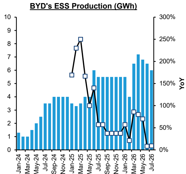
EXHIBIT 32: BYD – monthly production for ESS was 6.0GWh(9%YoY)
