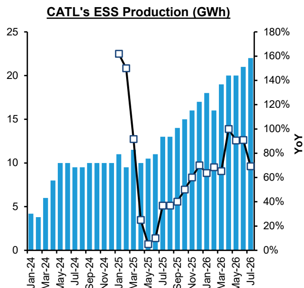
EXHIBIT 20: CATL - monthly production for ESS was 22 GWh(69%YoY)
