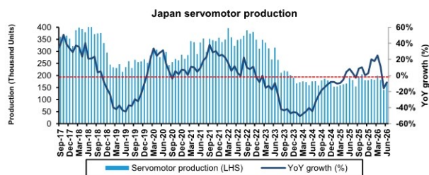
EXHIBIT 50: Japan - Servomotor production
