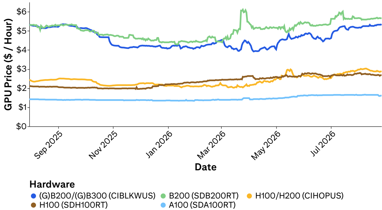
Figure 18. Rental Pricing for GPUs
