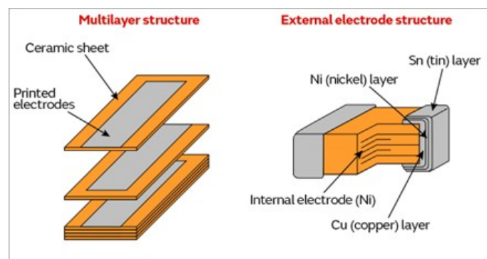
Exhibit 5: MLCC composition
