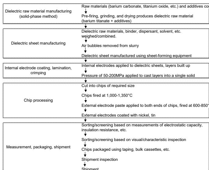
Exhibit 6: MLCC production process
