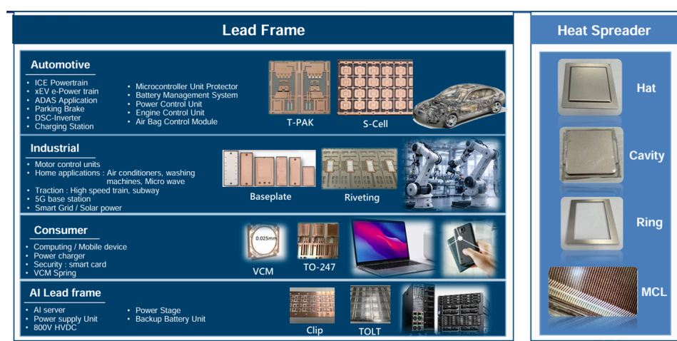
Fig. 7: SDI's electronic product offerings
