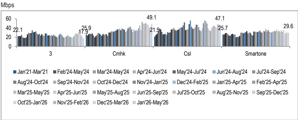
Figure 66: Hong Kong Southern: 4G download speeds
