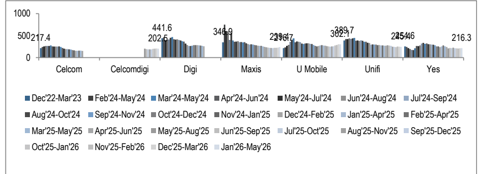
Figure 56: Malaysia Sabah: 5G download speeds
