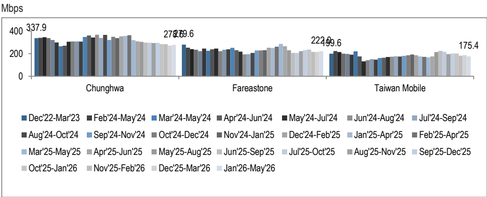
Figure 76: Taiwan Eastern: 5G download speeds
