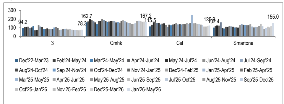
Figure 65: Hong Kong Southern: 5G download speeds
