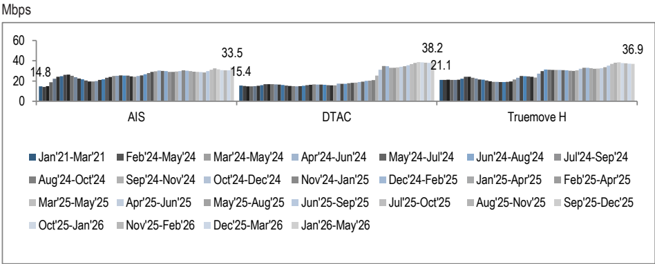
Figure 41: Thailand Bangkok: 4G download speeds
