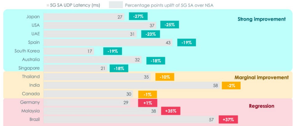
Figure 9: 5G SA typically reduces latency, but not uniformly
