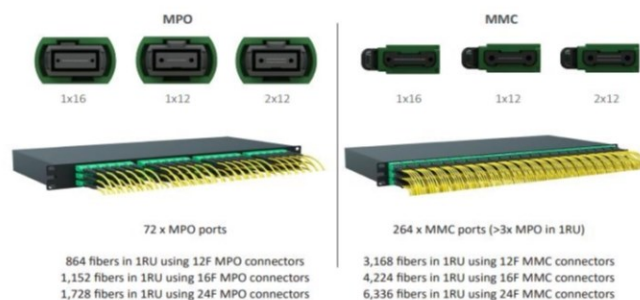
Fig. 2: MMC has a smaller footprint than MPO to enable a 3X optical interconnect density
