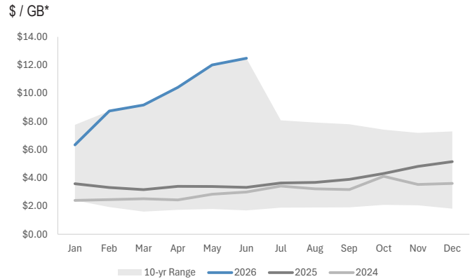
Figure 26: Monthly DRAM ASPs
