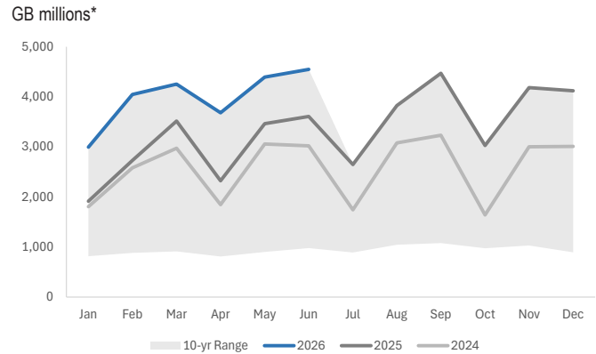
Figure 17: Monthly DRAM Bit Shipments
