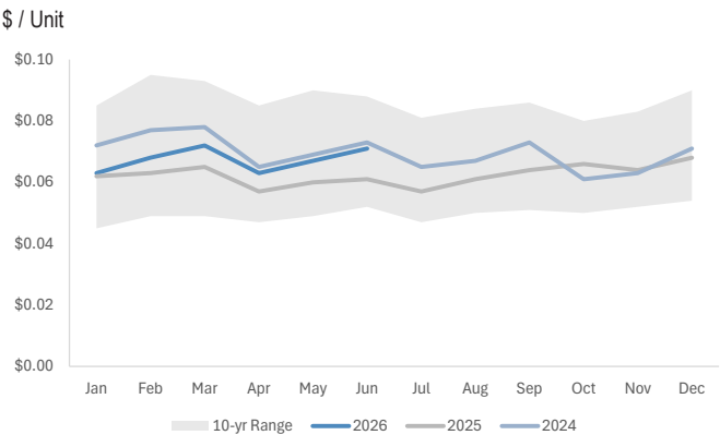
Figure 32: Monthly Discrete Devices ASPs
