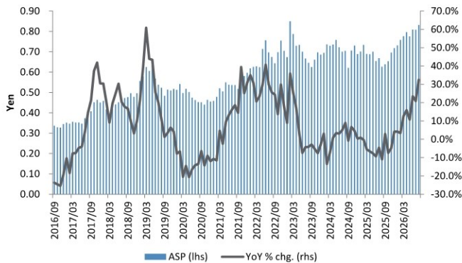
Figure 7: MLCC Export ASP (¥)
