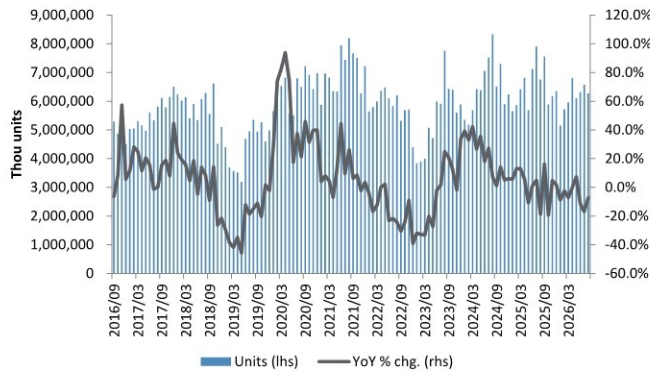
Figure 27: MLCC Export Quantity (thousands of units)
