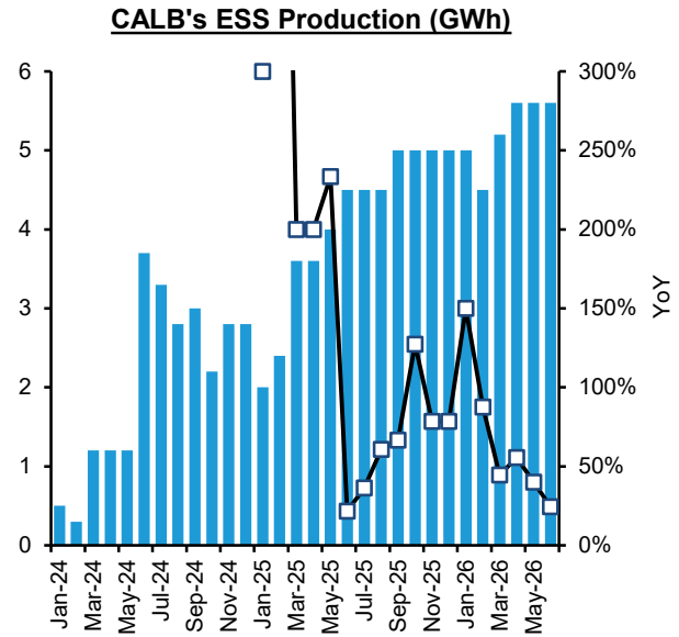
EXHIBIT 28: CALB - monthly production for ESS was 5.6GWh(40%YoY)
