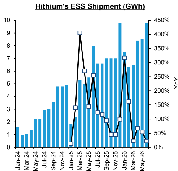
EXHIBIT 23: Hithium - monthly shipment for ESS was 9.8 GWh(23%YoY)
