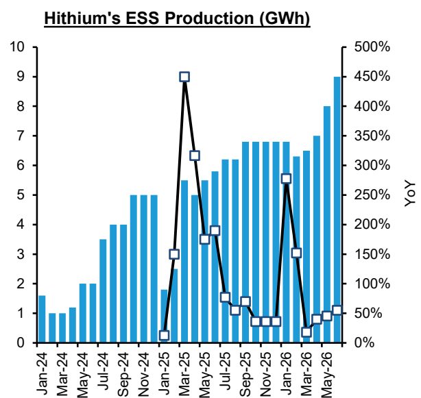
EXHIBIT 24: Hithium - monthly production for ESS was 9.0 GWh(55%YoY)
