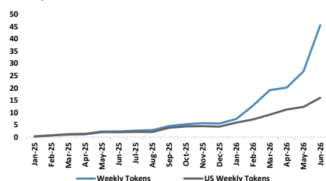
Figure 1: Token Volumes
