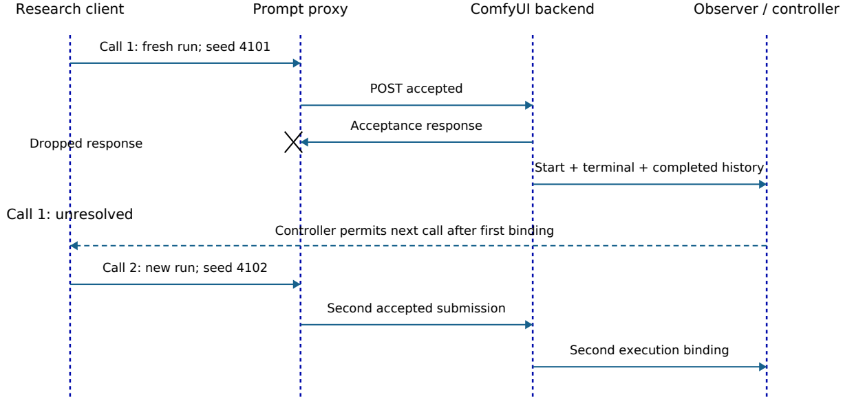
FIGURE 2. Controlled F02 protocol. The proxy hides the accepted response; backend observation gates a second call that creates a fresh run with a changed seed. Retained receipts and bindings support the two submissions and the ordering of the second receipt after the first retained binding. The campaign does not exercise the same-run guard. Spacing is schematic, not a measured latency or GPU-runtime plot.
