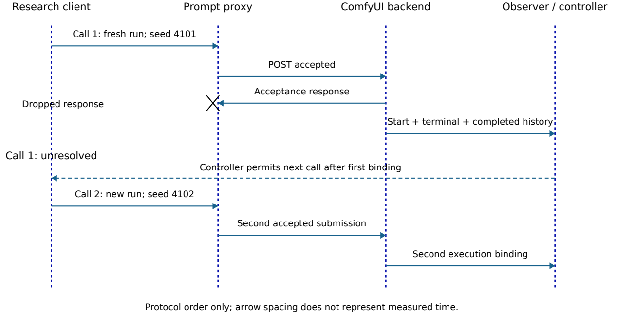
Fig. 2. Controlled F02 protocol. The proxy hides the accepted response; backend observation gates a second call that creates a fresh run with a changed seed. Retained receipts and bindings support the two submissions and the ordering of the second receipt after the first retained binding. The campaign does not exercise the same-run guard. Spacing is schematic, not a measured latency or GPU-runtime plot.
