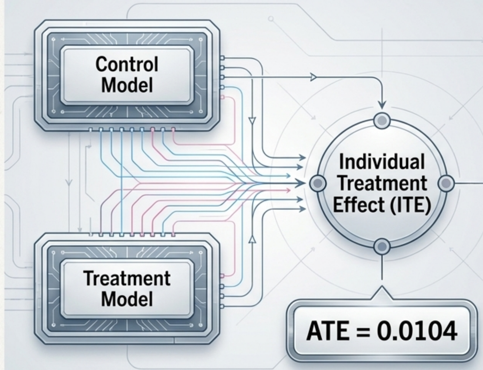
T-Learner Meta-Classfier
