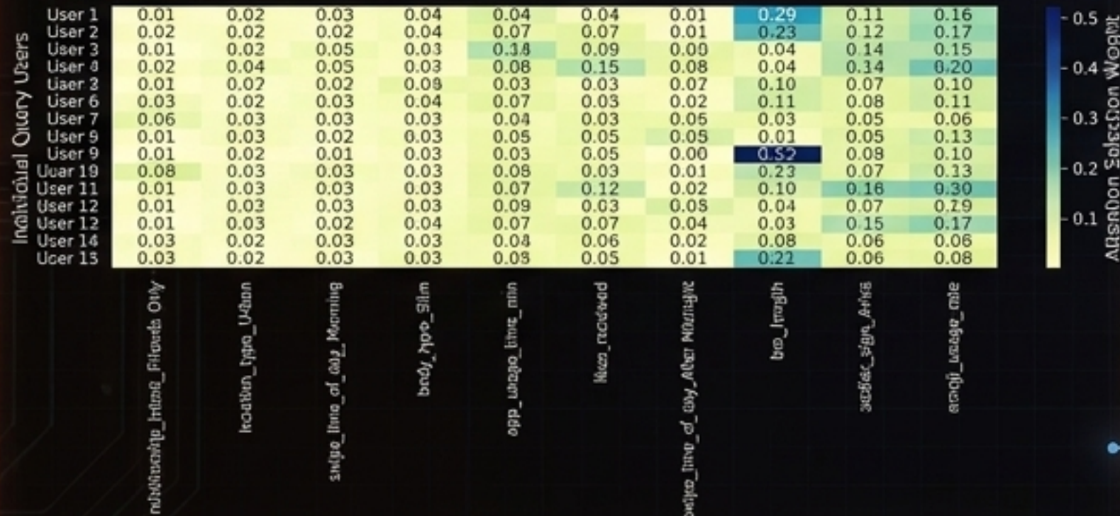
Instance-Wise Feature Selection Heatmap (Attentive Tabular Network)
