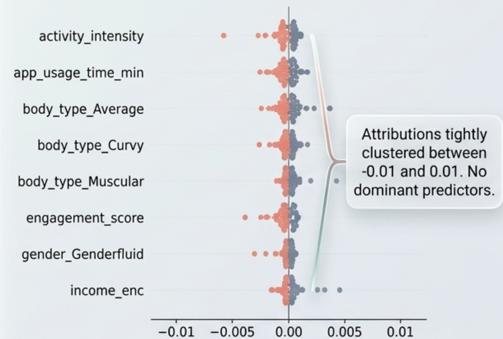
Global Impact: Predictive Void
