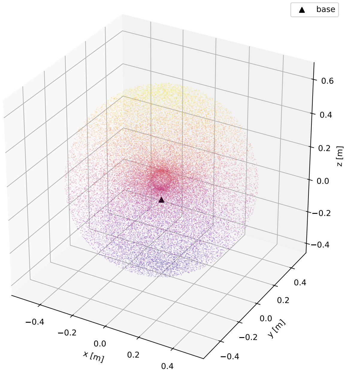
7-DOF reachable workspace (Monte-Carlo, std DH, 200,000 samples)
