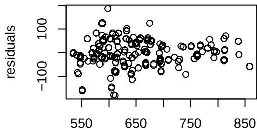
Resids vs. linear pred.
