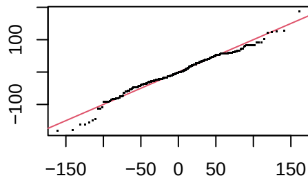
deviance residuals
