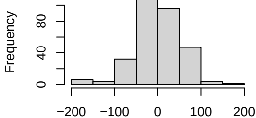
Histogram of residuals
