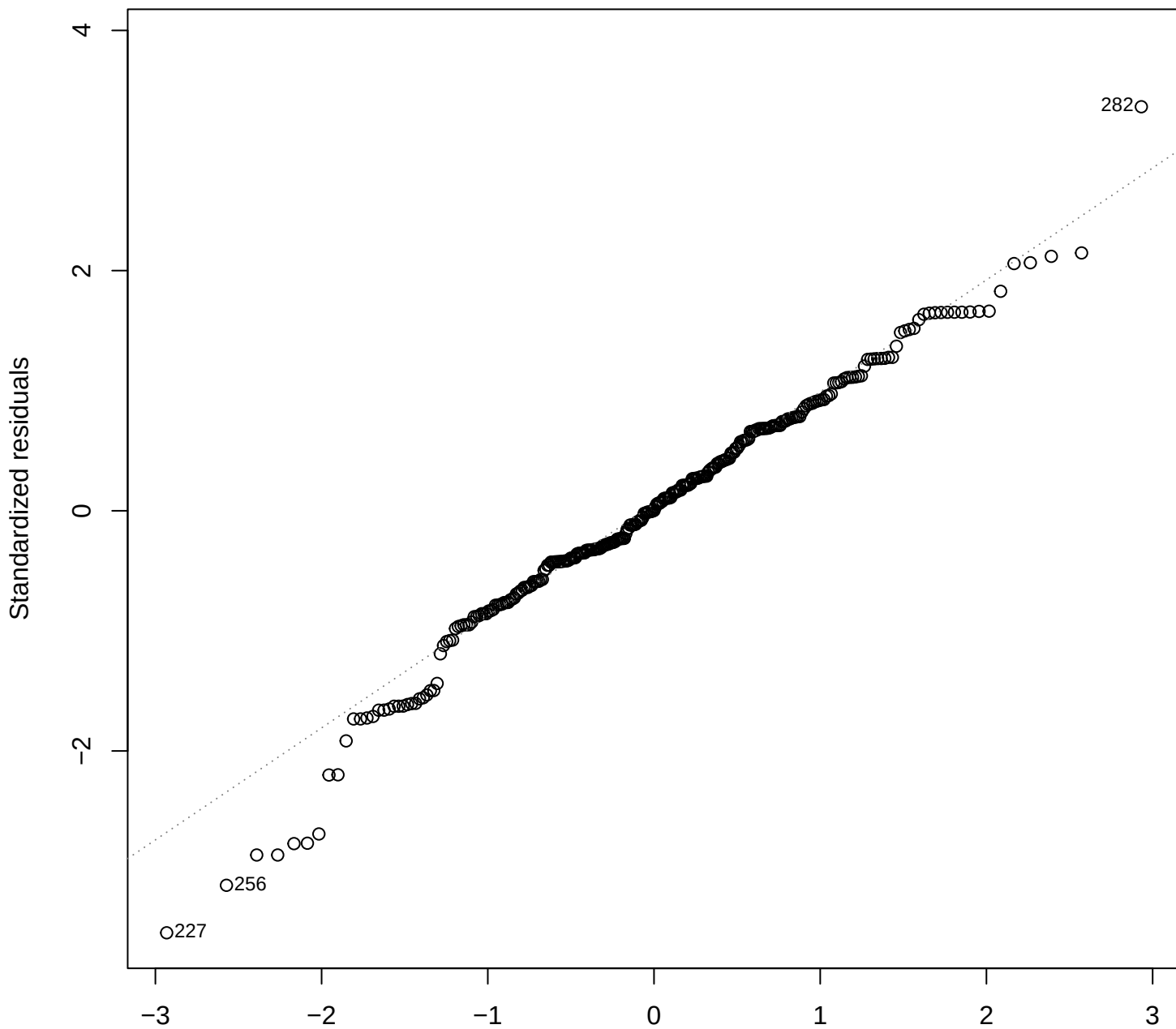
Q-Q Residuals
