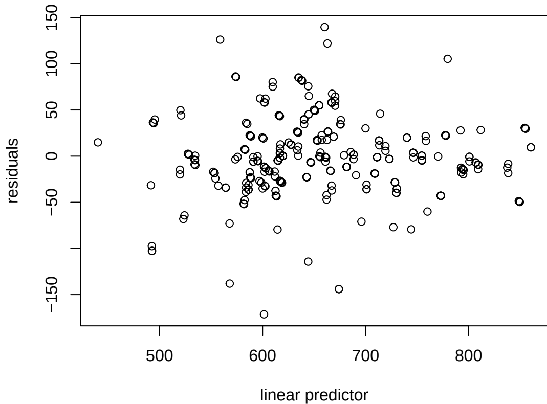
Resids vs. linear pred.
