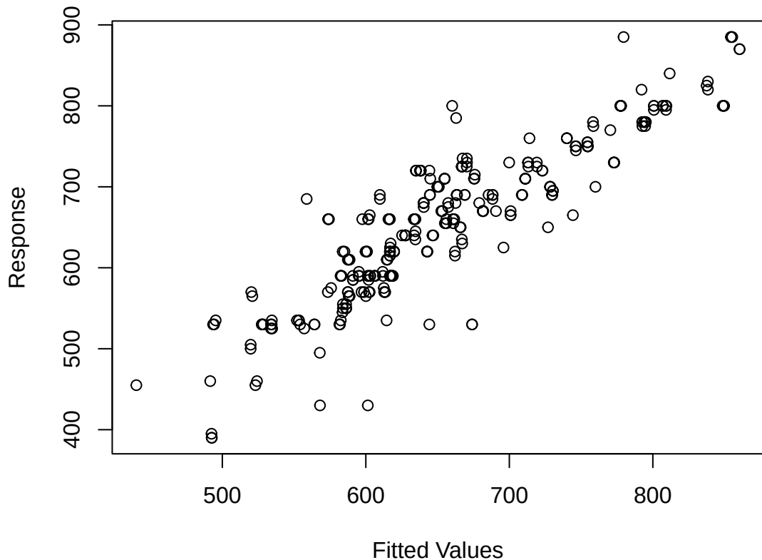
Response vs. Fitted Values
