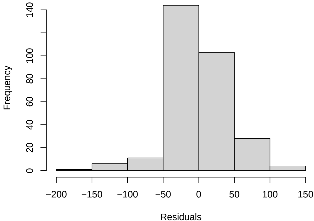
Histogram of residuals
