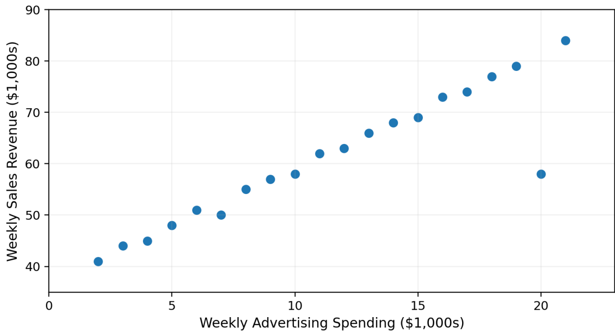
Figure 1. Weekly advertising spending and weekly sales revenue for 20 randomly selected weeks.
