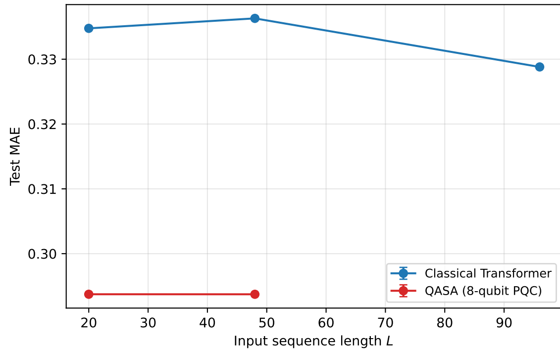
Chaotic Logistic
