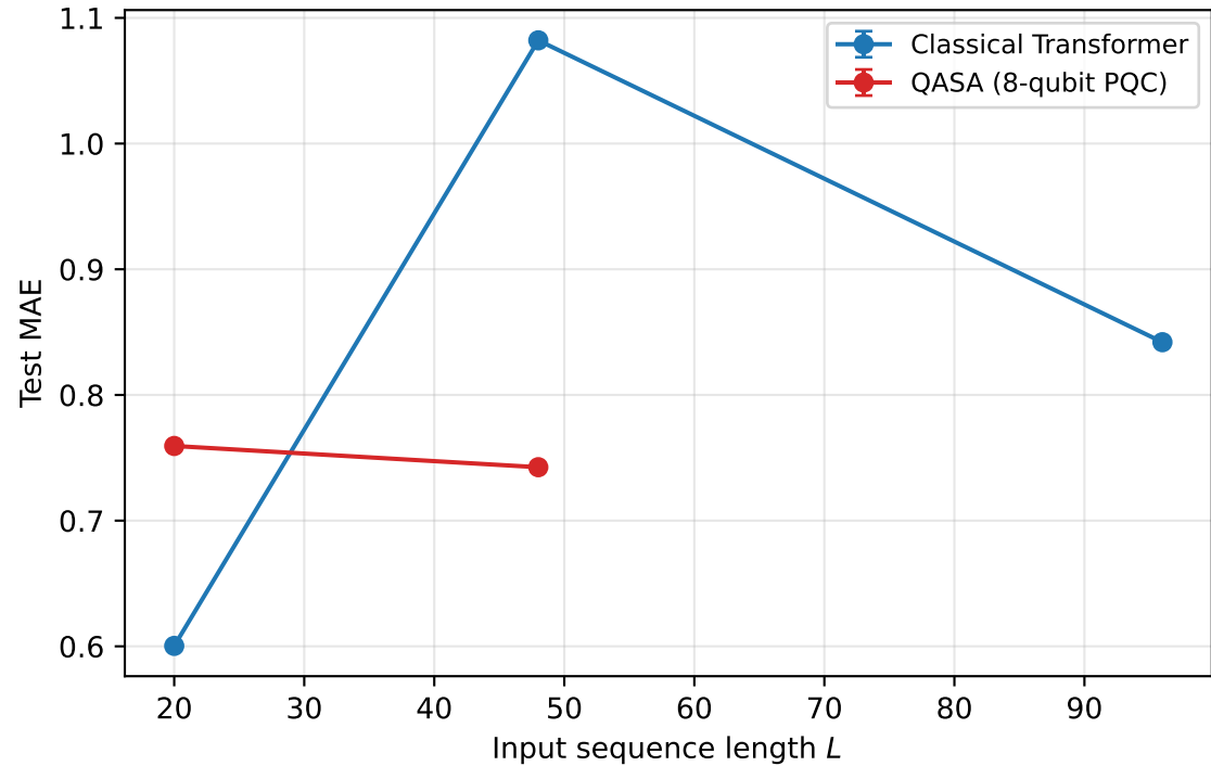
Seasonal Trend
