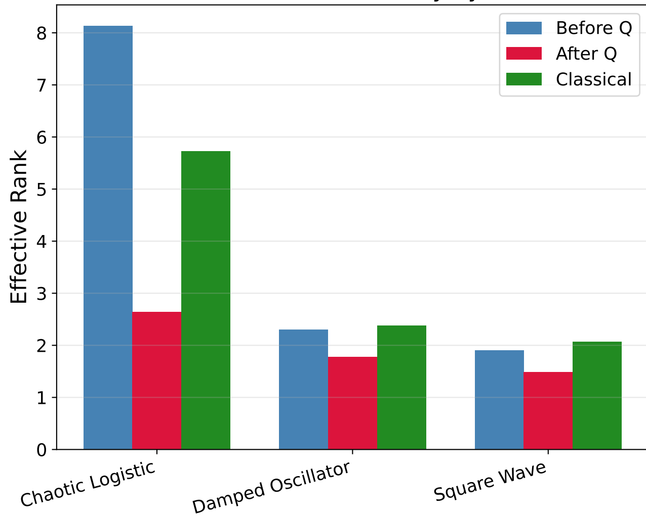
Effective Dimensionality by Task
