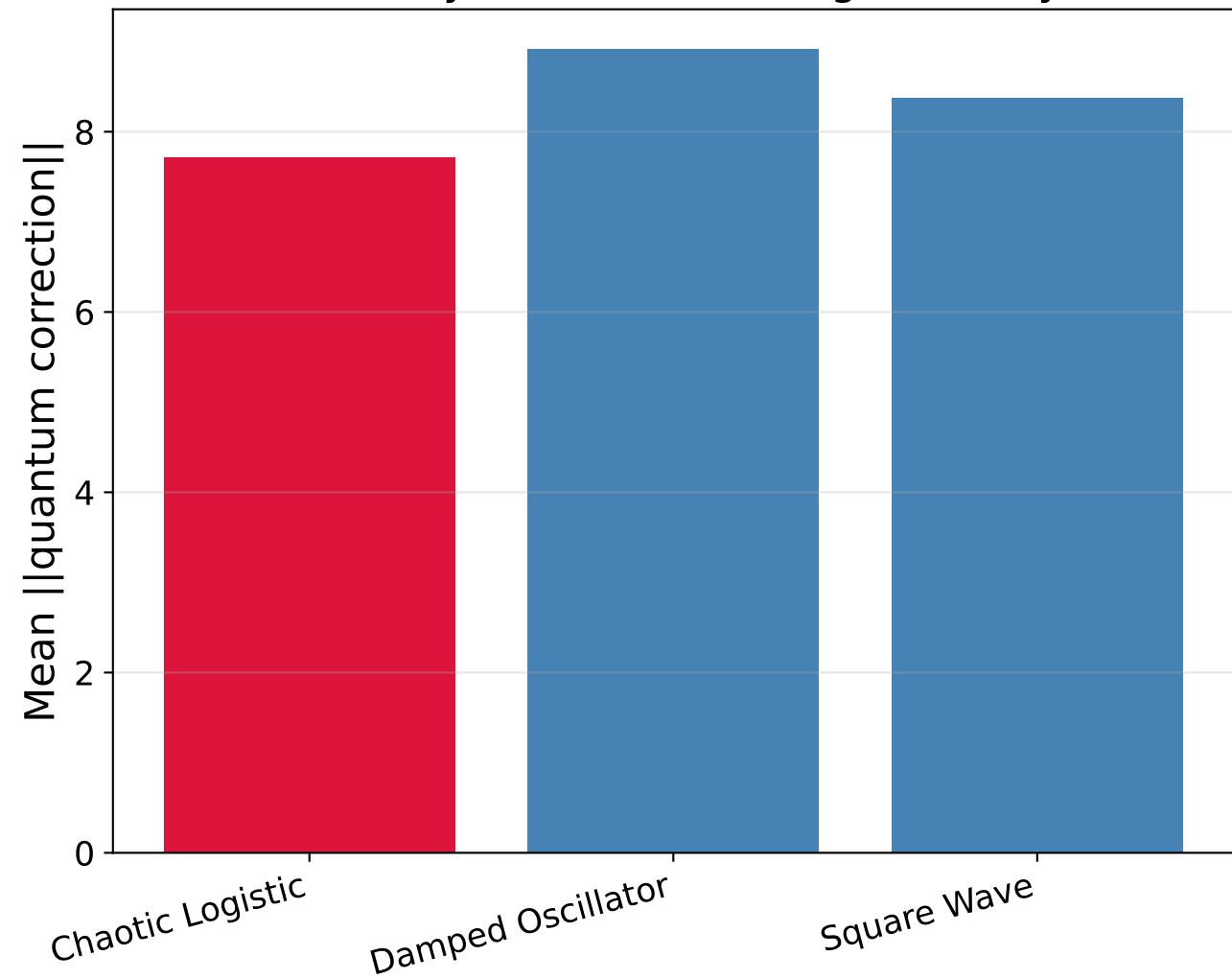
Quantum Layer Correction Magnitude by Task
