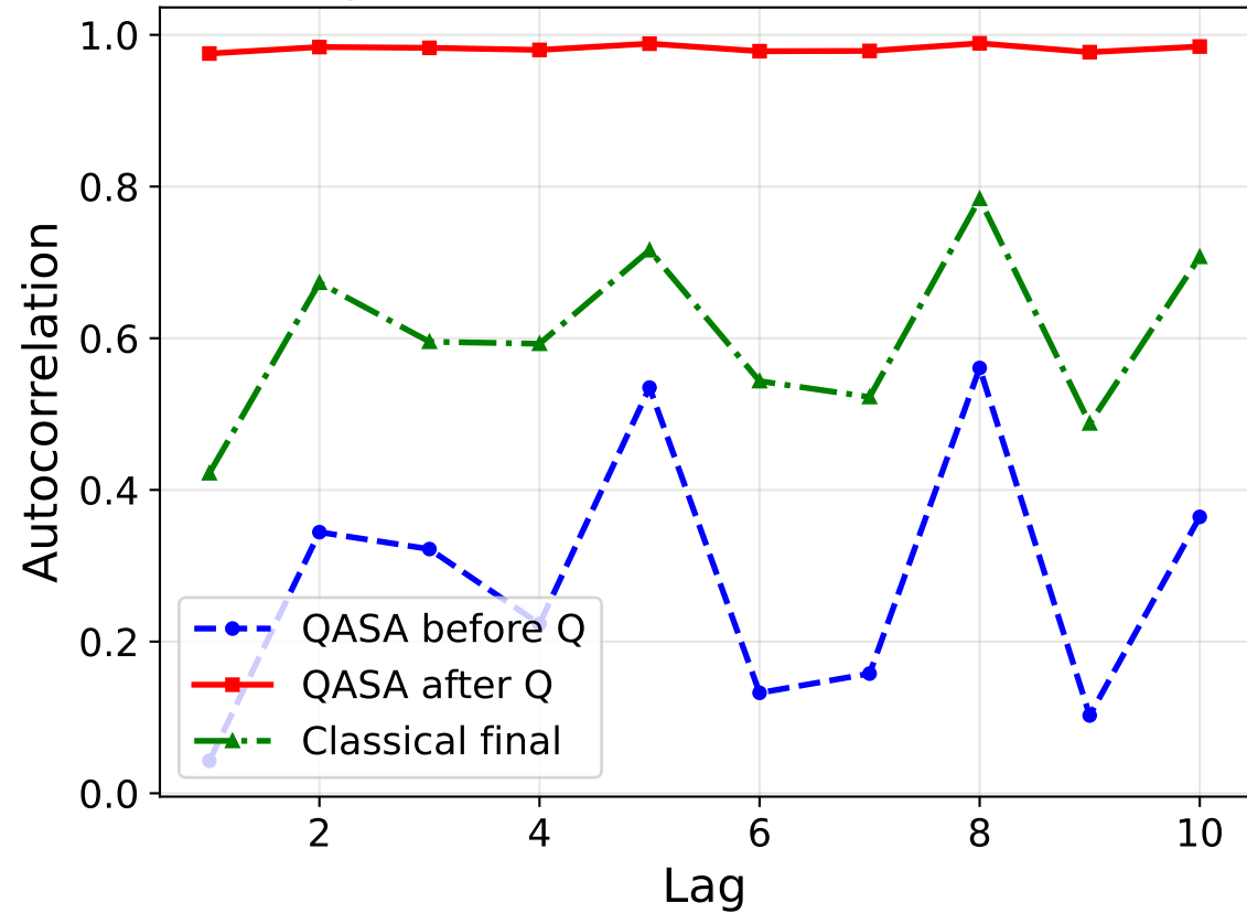
Temporal Autocorrelation of Features
