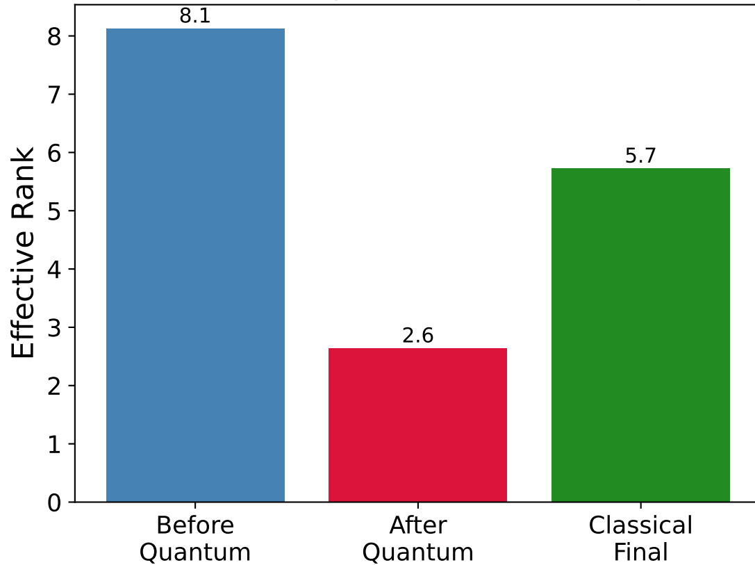
Feature Space Dimensionality
