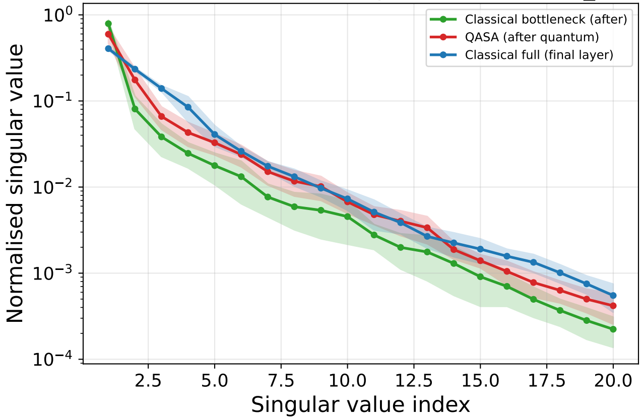
Bottleneck vs QASA vs full-classical spectrum: classical_chaotic_logistic
