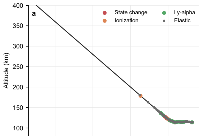
Single H ENA trajectory, 400 km/s, atmospheric segment
