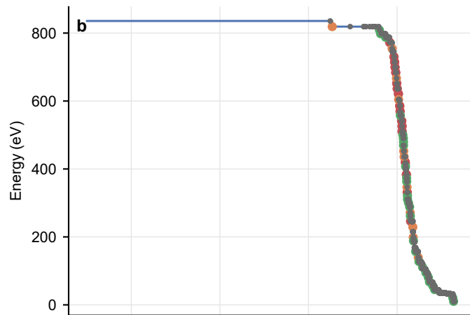
Single H ENA trajectory, 400 km/s, atmospheric segment
